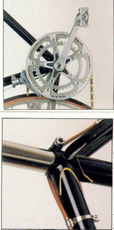
5-arm cotterless alloy cranks with inter-changeable inner and outer sprockets for easy gear ratio changes. Professional style aluminum pedals by MKS.
