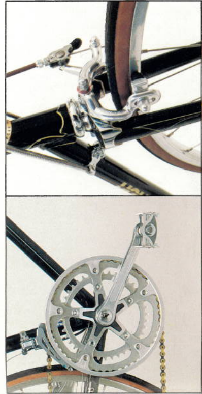
5-arm cotterless alloy cranks with inter-changeable inner and outer sprockets for easy gear ratio changes. Professional style aluminum pedals by MKS.
