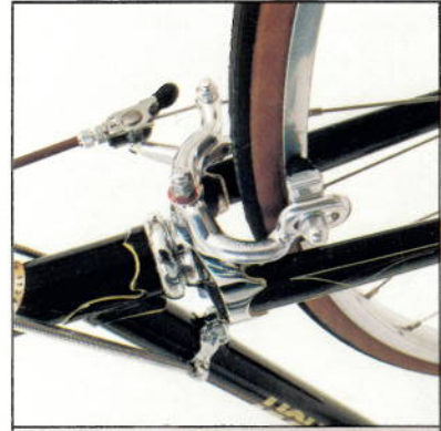
Dia-Compe 500-Q forged alloy side pull brakes with quick release mechanism. Advanced fork design for strength. Chromed crown for racy good looks. Centurion 27" 250 gram 25mm 100 psi skin tires for lightweight roadability.
