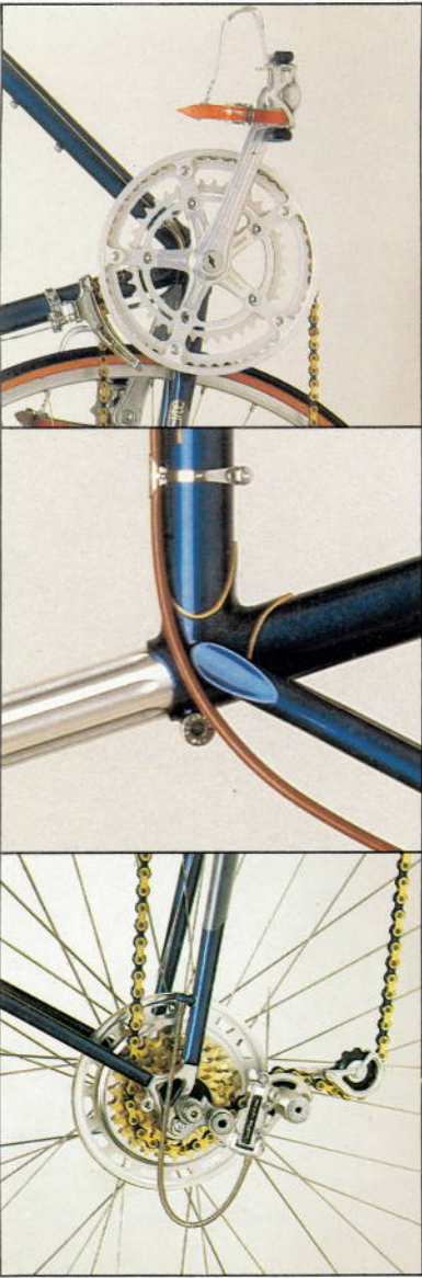
Suntour Cyclone GT Derailleur system with Suntour Tan-Z cluster and chain. Inner edges of chain's outer link plate are deeply scalloped; so chain operates at a sharper angle, engaging cluster teeth more quickly for greater shifting speed.
