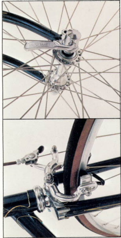
Suntour Vx small flange, quick release hubs, front and rear. Chrome forged fork end. Stainless steel spokes. Dia-Compe 500-G forged alloy side pull brakes, with quick release mechanism for extremely positive braking. Advanced fork design with chrome crown, 27" x 19.6mm alloy rims. Centurion high performance 27" x 250 gram 25mm 100 psi skin tires.
