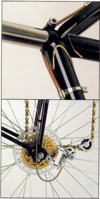
Suntour's new VX Derailleur system with gold Tran-Z chain and gold 6-speed freewheel. New cog design is as narrow as a normal 5-speed. Teeth are sharply tipped and "zigzagged" to fit each link plate precisely to enable quick, smooth speed changes.
