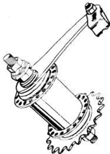
"Sun Tour" Coaster Hub
