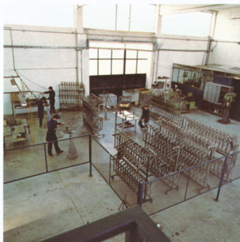
Reparto squadratura e limatura Squaring and filing department Endmontage Atelier de dressage et limage
