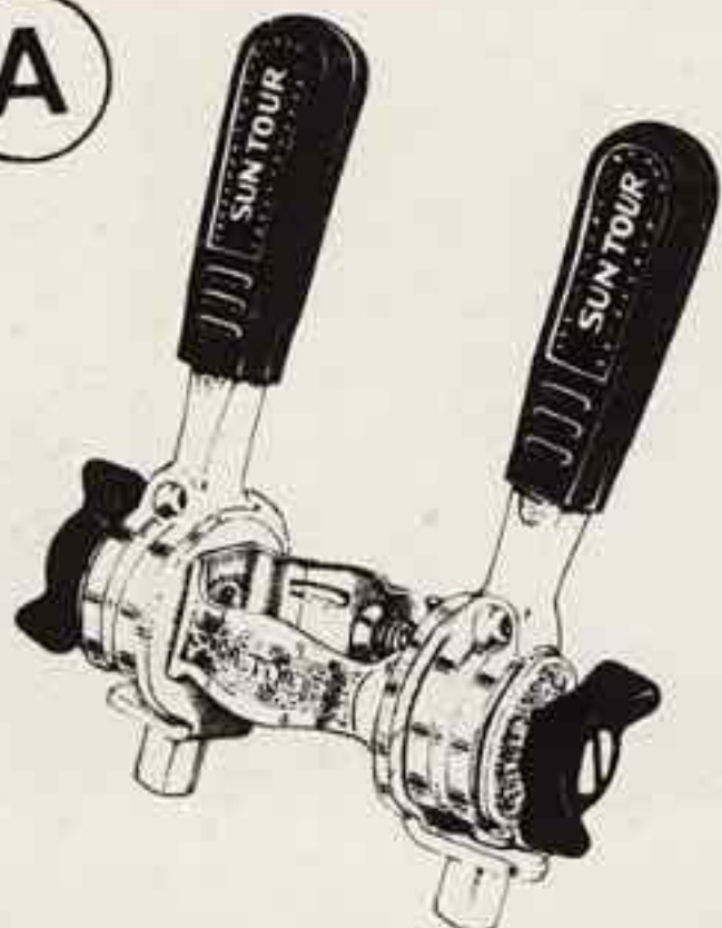
SUNTOUR DOUBLE LEVER No.3302 DLW
