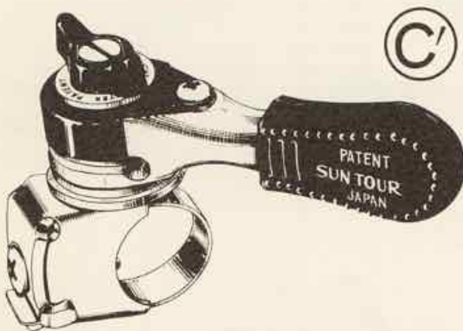
SUN TOUR MIGHTY SHIFTER No. 3450 Sun Tour Power single lever For 7/8" tubes 15/16" tubes
