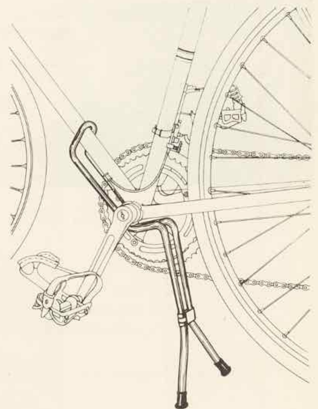
SUNTOUR MULTI-STAND No.4500
