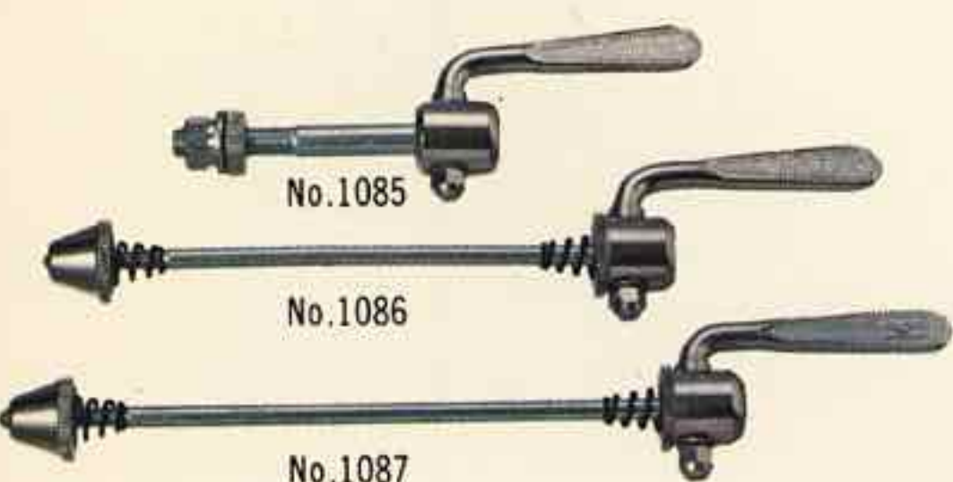
No. 1085 QUICK RELEASE FOR SEAT PILLAR No. 1086 QUICK RELEASE FOR FRONT HUB No. 1087 QUICK RELEASE FOR REAR HUB
