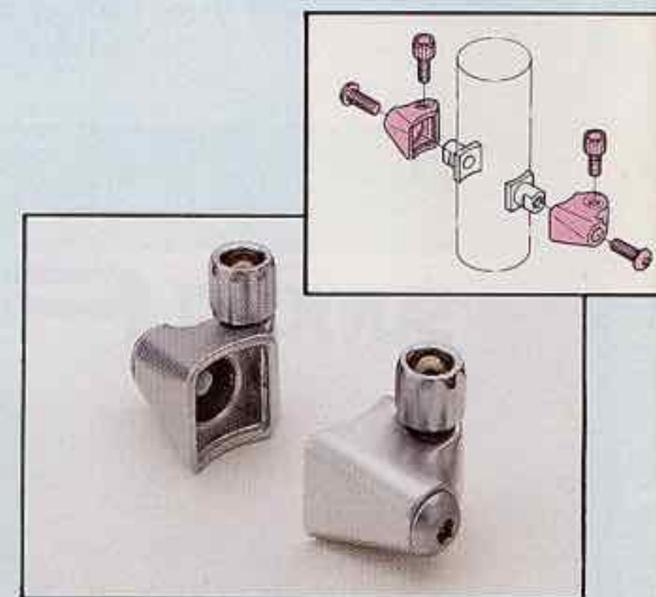
CABLE CASING STOP Model: OS-410 (Code No.55310211) Right (Code No.55310212) Left Specifications ● Material: Aluminum alloy (Body) Steel (Mounting bolt & adjuster) ● Use: Downtube casing stop
