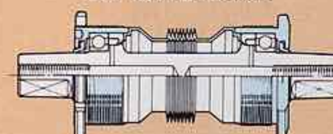
BOTTOM BRACKET
