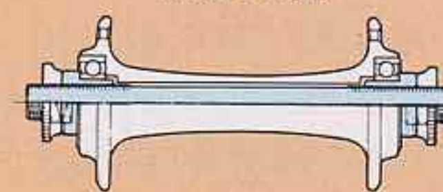
FREEHUB
