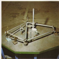
Truing plate for every frames
