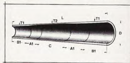
Cut-away view of a double-butt tube
