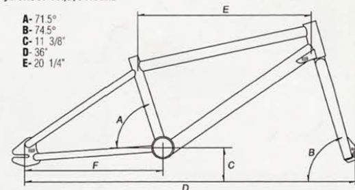
'92 GROUP 1 A, B, C FRAME
