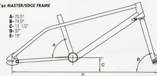
'92 MASTER/EDGE FRAME
