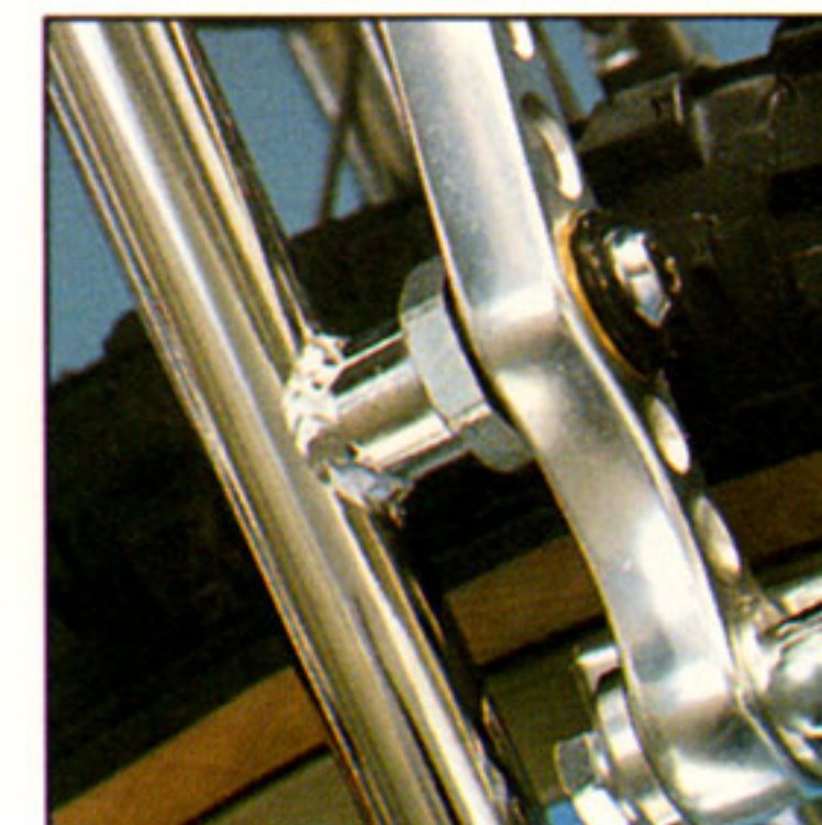
Heliarc welded cantilever mounts are more reliable than brazed-on mounts.
