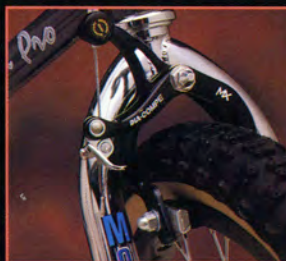
Dia Compe side pull brakes have quick release feature for easy wheel removal.
