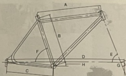
FRAME GEOMETRY
