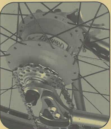
ROHLOFF SET-UP
