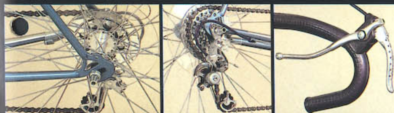
1 - MAILLARD HUB WITH ALLEN FAST RELEASE NUT, SEMI-FORGED TIP AND BRAZED-ON CABLE STOP. - 2 - SUN TOUR AR DERAILLEUR WITH MAILLARD 6 COGS SILVER FREE WHEEL AND SEDISPORT CHAIN. - 3 - RANDONNEUR BAR FEATURES EXCLUSIVE MOTOBECANE SLEEVES; DRILLED ALLOY BRAKE LEVERS WITH DUAL CONTROL.
