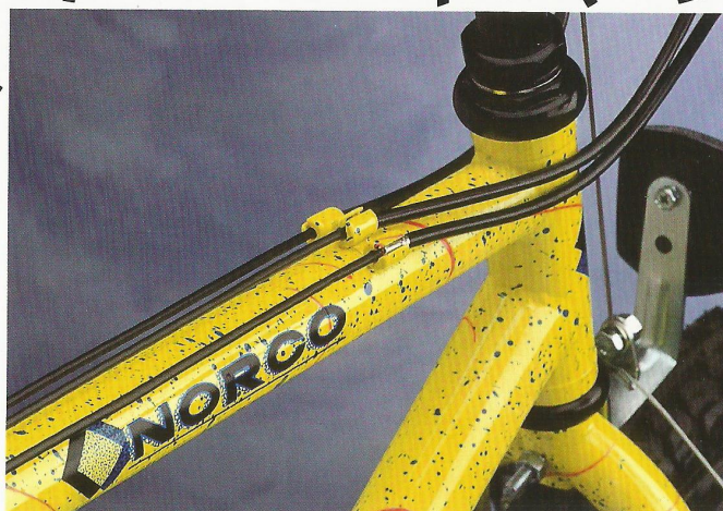
Top-tube mounted open cables reduce friction in the front and rear changer cables and result in increased power to the rear brake by reducing casing compression.
