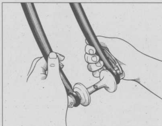
IT SHOULD REQUIRE FIRM PRESSURE TO CLOSE THE LEVER COMPLETELY. NOTE THE GRIP AND THE FINISHED LEVER POSITION. DO IT RIGHT!
