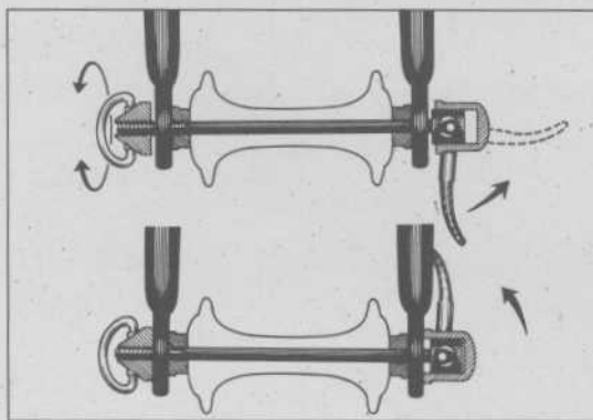
THE Q/R LEVER OPERATES A CAM. TENSION IS REGULATED BY THE OPPOSITE-SIDE NUT/CONE.
