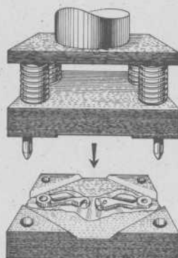
...THEN SMASHED TWICE. IN THIS CASE, THE SECOND AND FINAL SMASHING COMPLETES THE SHAPE.
