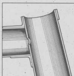
CAPILLARY ACTION DRAWS MOLTEN BRASS INTO THE TUBE/LUG GAP.
