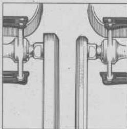
LEFT: MELT-FORGED CRANKS ARE THICK, INCREASING Q . RIGHT: COLD-FORGED CRANKS ARE SKINNY, KEEPING Q LOW.
