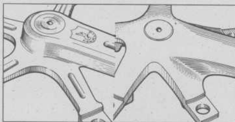
LEFT: COLD-FORGED CRANK TYPICALLY HAS SMALLER RADIUS, LOWER Q . RIGHT: MELT-FORGED CRANK HAS LARGE RADIUS, INCREASING Q .
