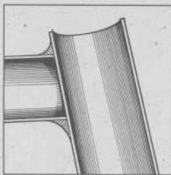
MOLTEN BRASS FLOWS INTO AND AROUND THE JOINT.
