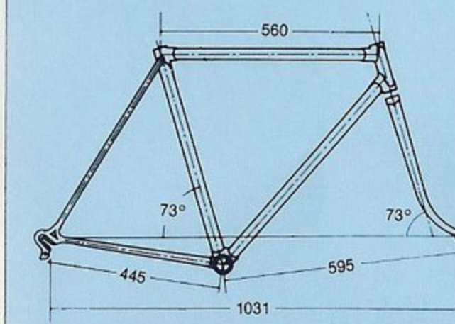
TOURING DX 23" (585mm)
