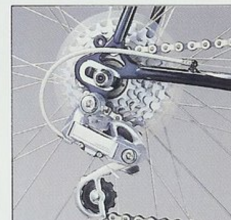
Shimano Z505 rear derailleur and Shimano 600UG silver freewheel.
