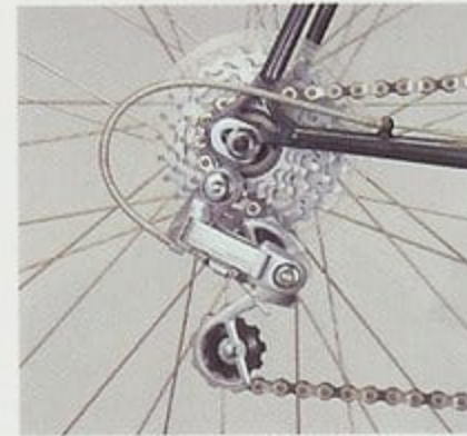
Shimano Z505 rear derailleur and Shimano 600 UG silver 6 speed freewheel.
