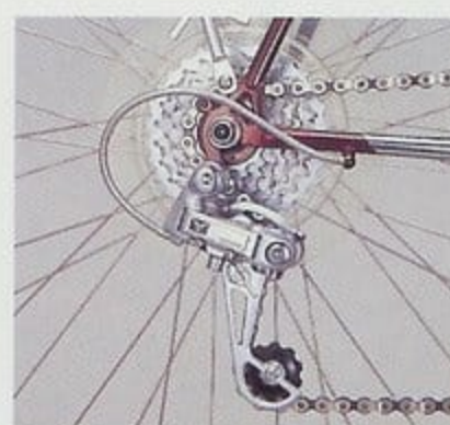
Shimano Deore XT Super Plate rear derailleur, Shimano 600UG silver 6-Speed freewheel and forged rear ends.
