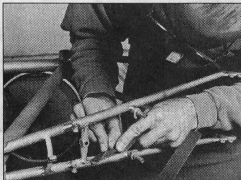
Curt files the edge of a non-essential seat stay bridge reinforcement.
