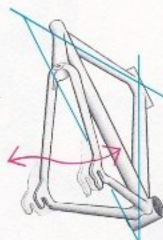
THE 5000 ALUMINUM—STIFFER IN OUT-OF-PLANE BENDING AND TORSION THAN CONVENTIONAL ALUMINUM BONDED FRAMES
