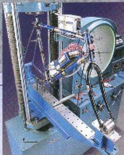
Schwinn's "Robo Bike" test lab re-creates actual riding conditions using physical, mathematical, and Finite Element Analysis models.
