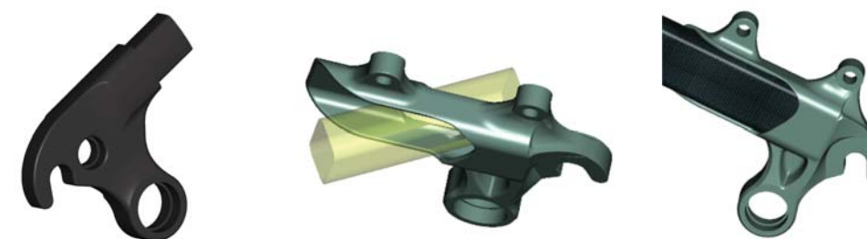
The FACT carbon dropouts and seatstays on the top-rung Stumpjumper FSR models are 20% lighter than their aluminum counterparts.
