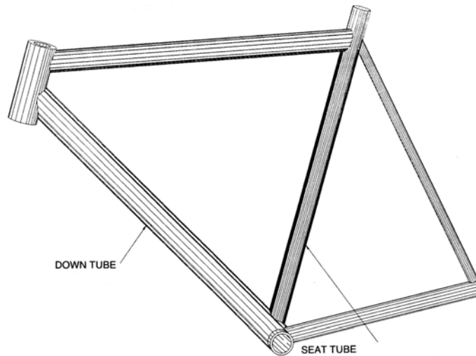
Figure 2. Bicycle Frame
