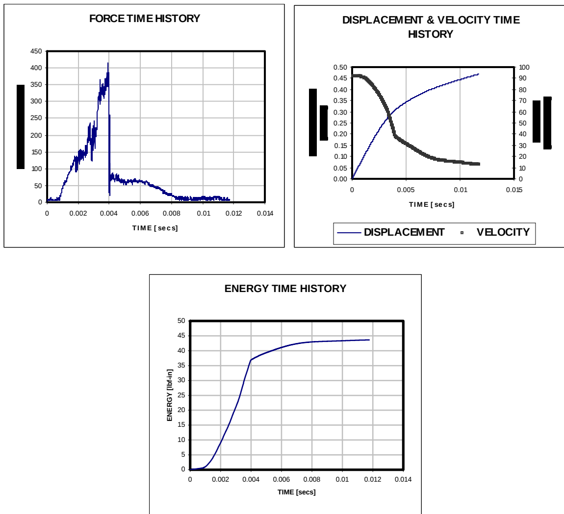
Figure 9. Force, Velocity and Impact Data
