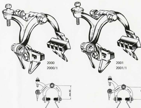
2000 Front caliper 2000/1 Front caliper ( short-reach)
