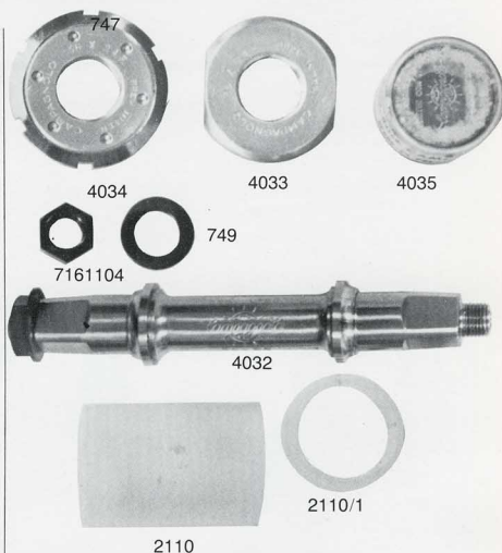
Super Record Road 4031
