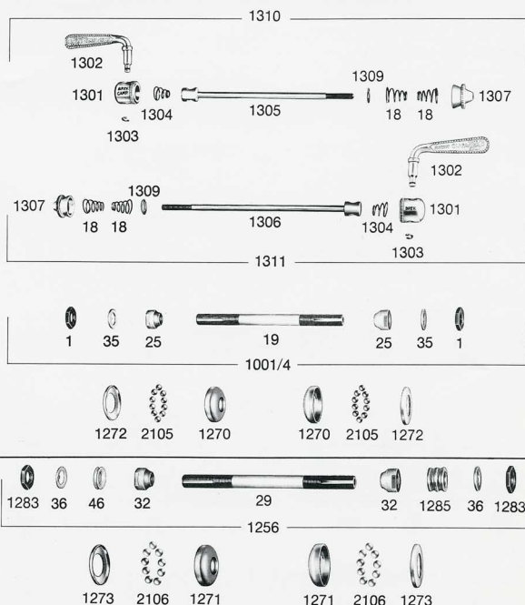
Gran Sport Hub parts
