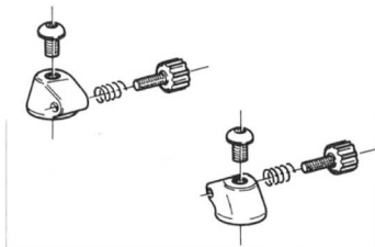
ERGOPOWER BLOCKS FOR ALUMINIUM FRAME
