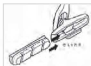
NEW PAD COUPLING/ UNCOUPLING SYSTEM: Easier pad replacement - greater safety.
