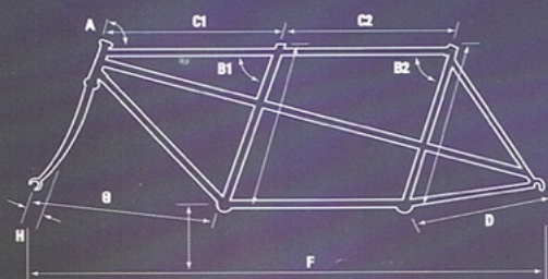
Frame Geometry
