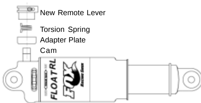
Fig. 1 Adapter Plate, Spring and Lever Installation
