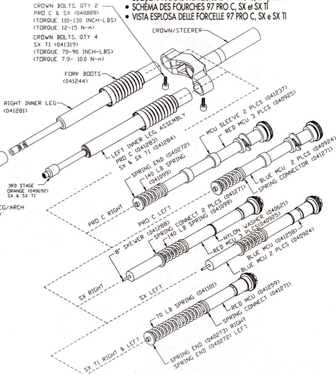
FIGURE 9: • 97 PRO C, SX & SX TI FORK SCHEMATIC
