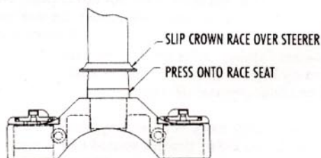
FIGURE 2: Race installation
