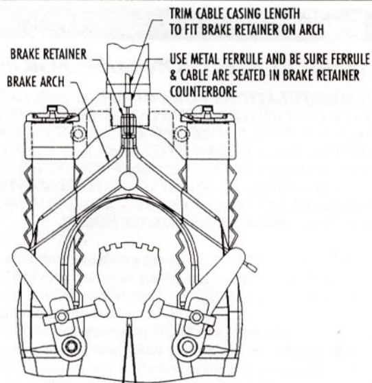
FIGURE 3: Brake cable routing
