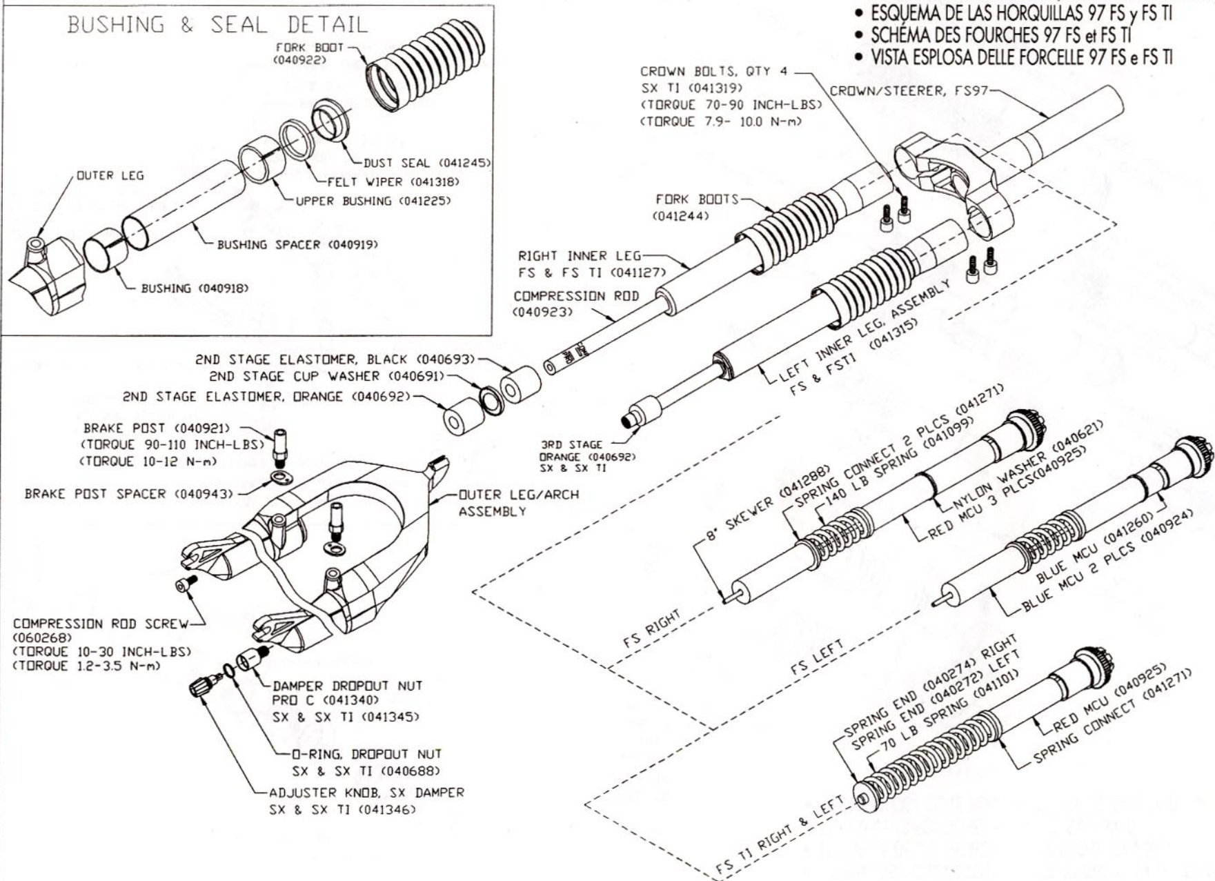
FIGURE 10: • 97 FS & FS TI FORK SCHEMATIC
