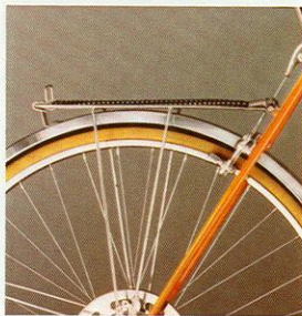
Rear carrier with sandow straps.
