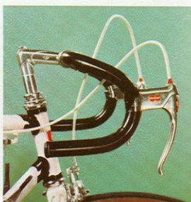
Racing handlebar with Altenburger special handles.
